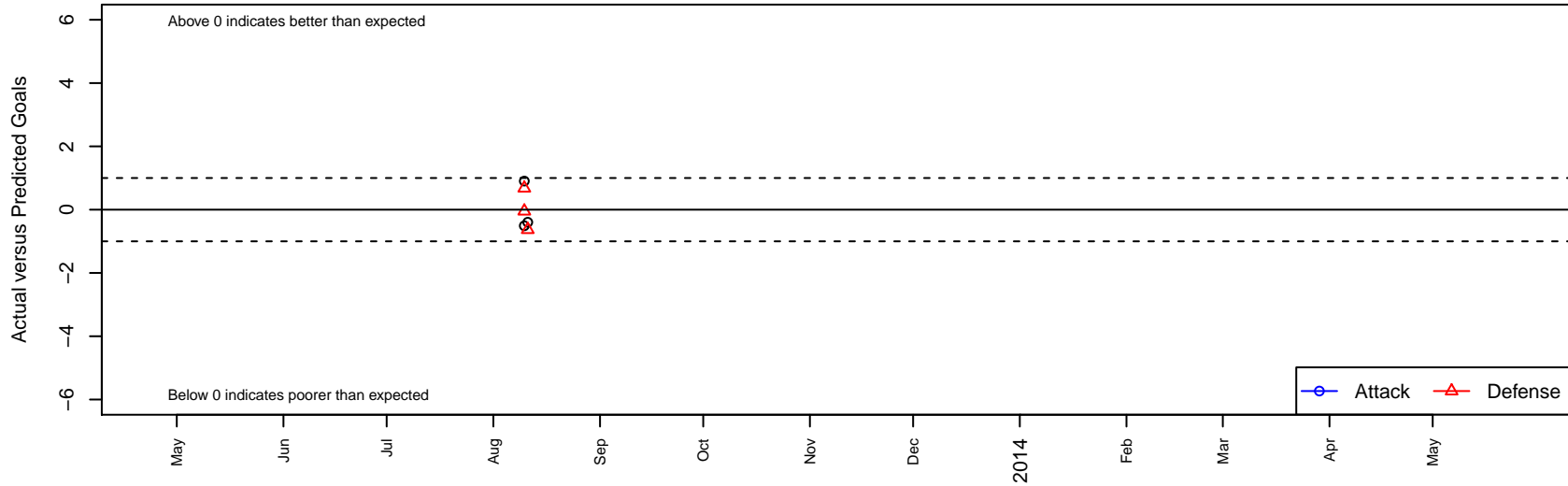
Encinitas Express Soccer White G99 Dots are actual minus expected GF (blue circles) and GA (red triangles). Blue line is smoothed change in attack strength. Red is smoothed change in defense strength.
